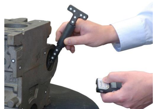
Touch Probe Accessory for Touch probing of hidden areas
